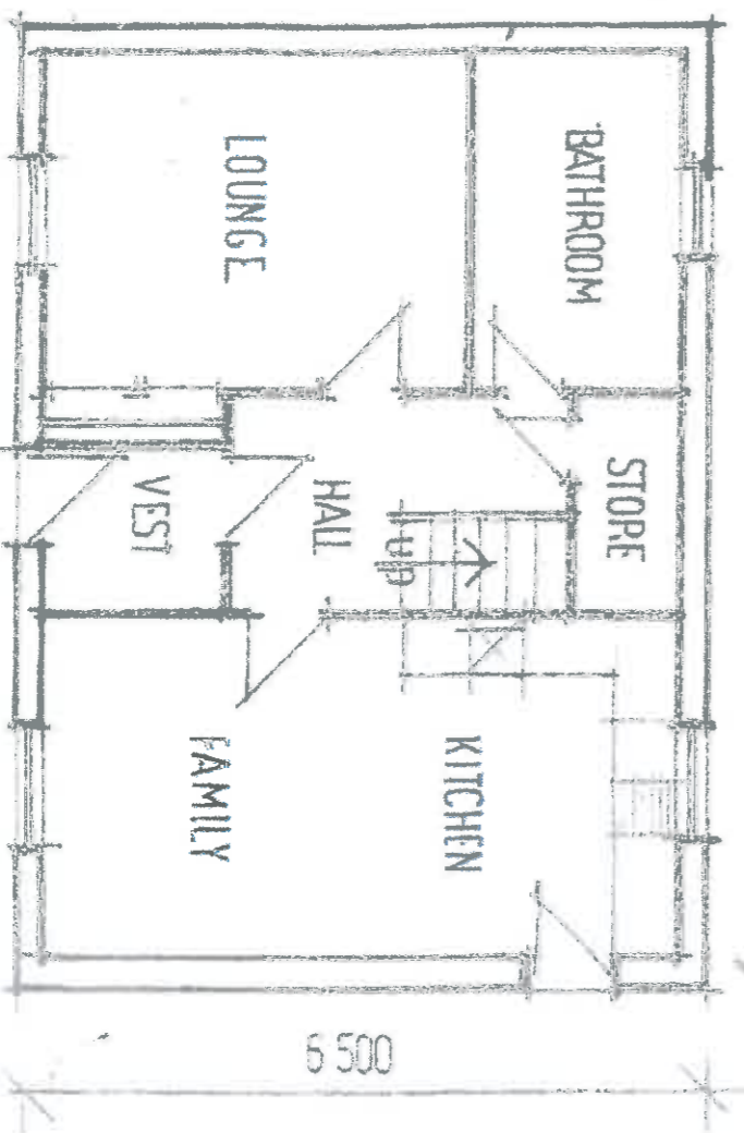
GROUND FLOOR 1:100
